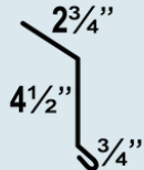
Eaves Flashing
