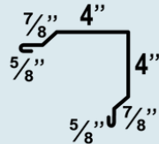
End Wall
