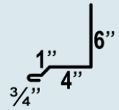
Side Wall
