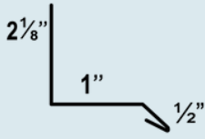
Base Trim
