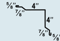
4" Inside Corner
