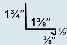
Drip Cap
